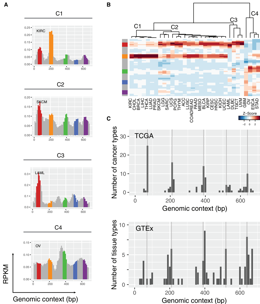
Figure 2. Recurrent eRNA Expression Peaks in Super-enhancers
