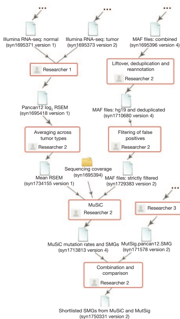
Figure 3 Example provenance graph of a multistep workflow showing interaction between the analysis of three researchers. The provenance record consists of two types of nodes—activities (shown as red boxes above) performed by a researcher and input and output files of these actions (shown as file and folder icons and identified by their name and Synapse ID). In addition, every activity has metadata associated with it to further describe the details of the actions performed. This specific graph shows the workflow used to perform comparative analysis of two mutation-calling algorithms—MuSiC and MutSig. For MuSiC, the provenance of analysis is displayed from input data to derivation of mutation calls. Provenance records may be further expanded (ellipses) to trace the origin of input files to their original data source in Firehose, DCC or personal communications with AWG members. For brevity, the MutSig graph is not expanded. This graph was produced from version 2 of the data in doi:10.7303/syn1750331 .
