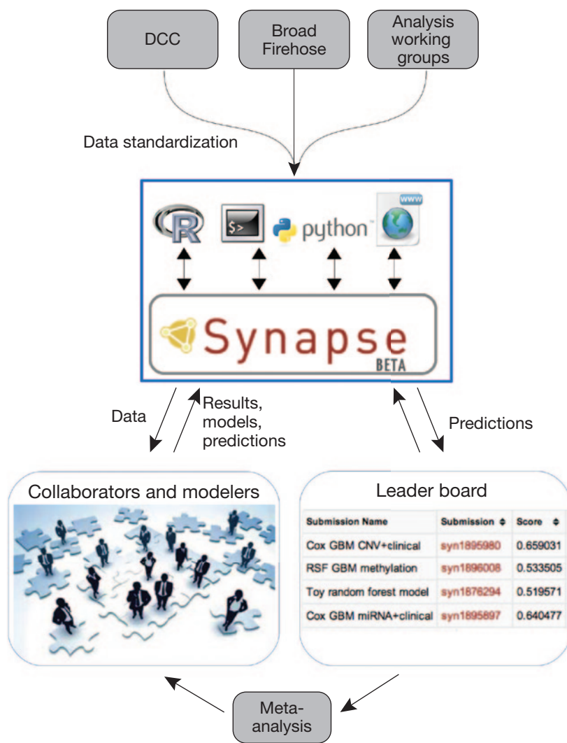
Figure 2 Schematic of the Pan-Cancer analysis workflow. Data were aggregated and standardized from the TCGA DCC, Broad Firehose and individual analysis working groups and processed into easy-to-use tab-delimited files. Collaborators used a variety of analytic tools, such as R, Python, Unix shell and the web client, to interact with data in Synapse while also storing results, provenance records, analysis descriptions and source code. For a subset of these results (for example, patient survival predictions), Synapse carried out automated performance evaluations and displayed results on a real-time leader board, which were available to collaborators to perform comparative meta-analysis or adapt model source code to additional applications.
