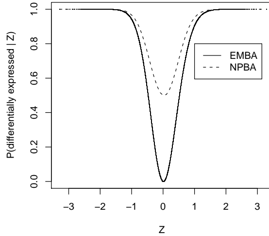
Figure 7: Estimated curve \overline{P}_1(z) under both, the EMBA and the proposed nonparametric Bayesian approach, for the Alon colon cancer data. The lower estimate under the EMBA is a direct consequence of the overestimated \widehat{p}_0 .
