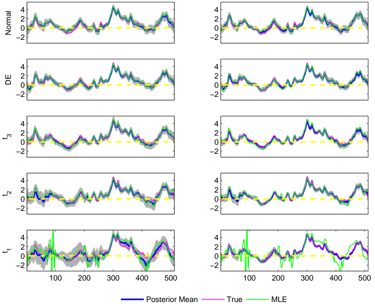
The estimated B_1(t) for 5 simulated datasets, simulation run 1
