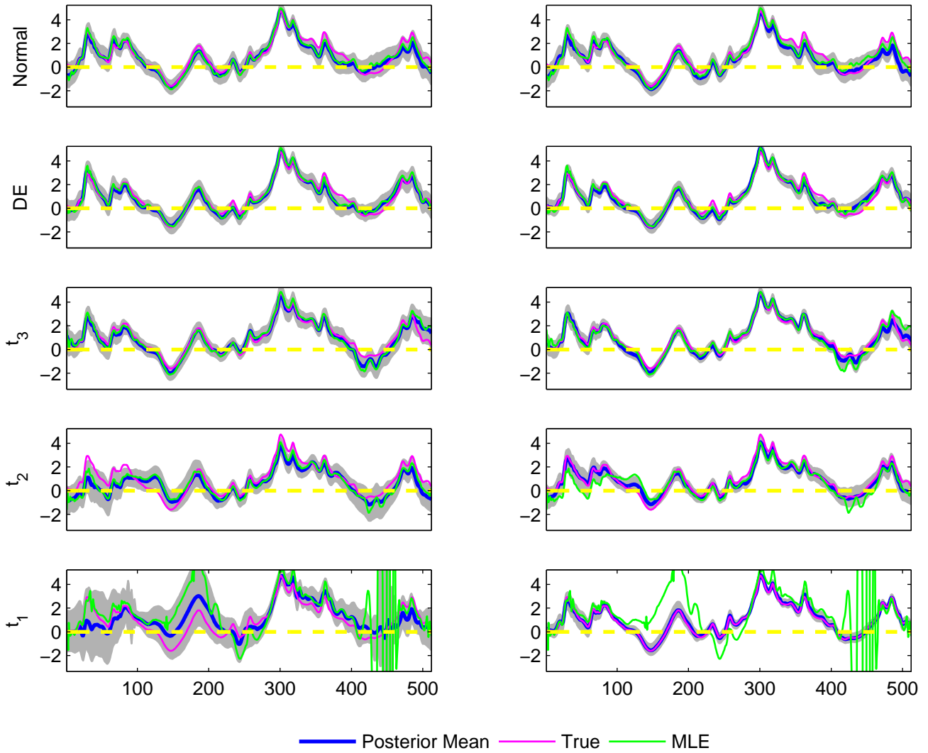
The estimated B_2(t) for 5 simulated datasets, simulation run 1
