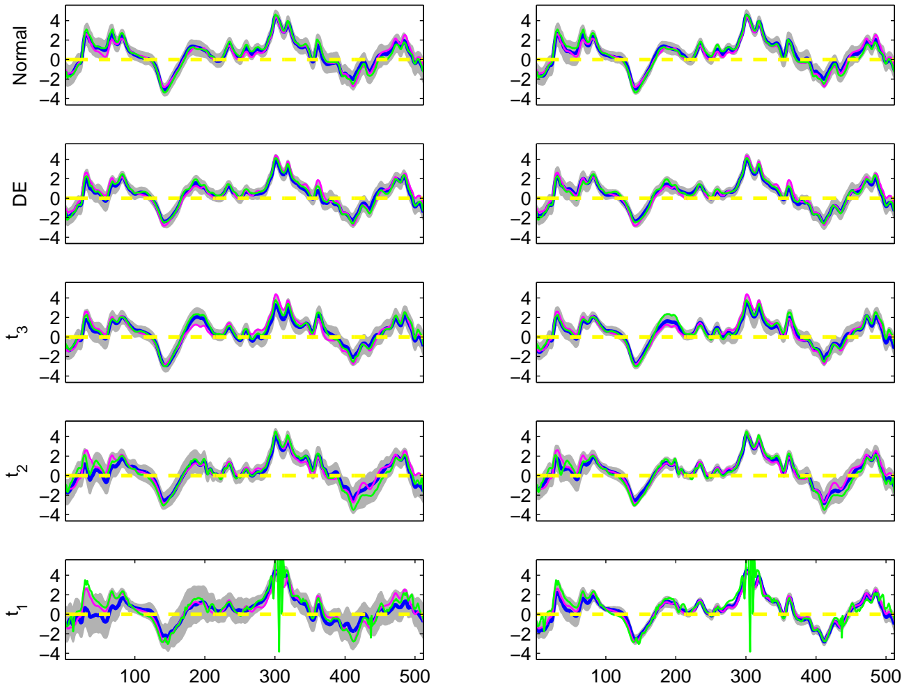
The estimated B_3(t) for 5 simulated datasets, simulation run 1
