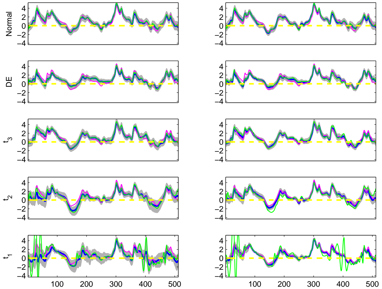
The estimated B_4(t) for 5 simulated datasets, simulation run 1
