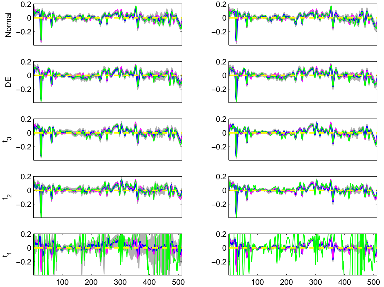
The estimated B_5(t) for 5 simulated datasets, simulation run 1
