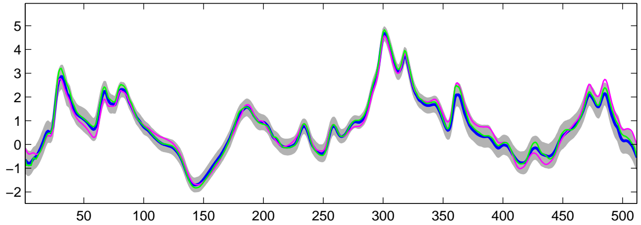
Estimated C_0(t) using G-WFMM: Normal data, run 1
