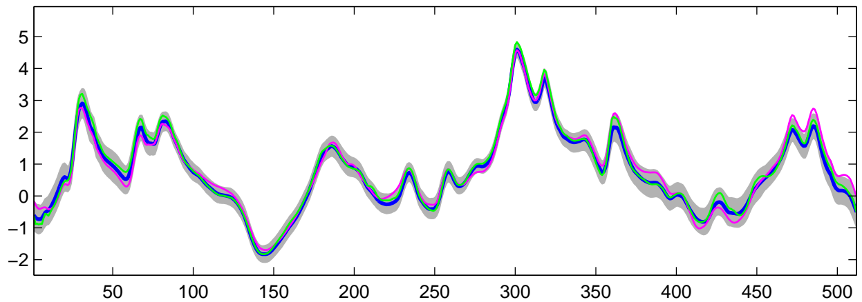
Estimated C_0(t) using R-WFMM: Normal data, run 1
