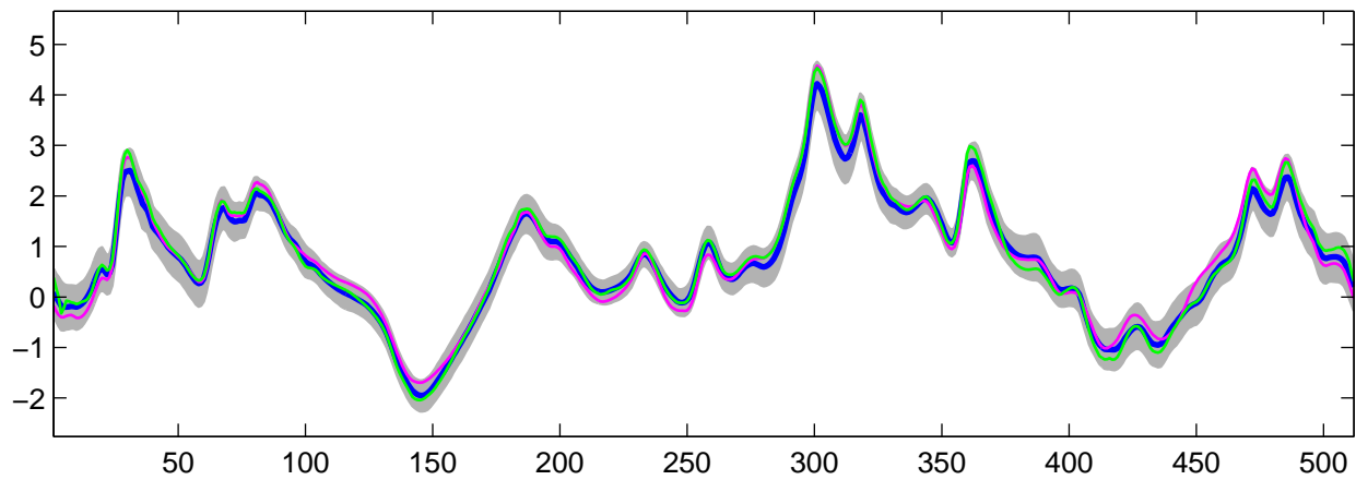
Estimated C_0(t) using G-WFMM: t_3 data, run 1
