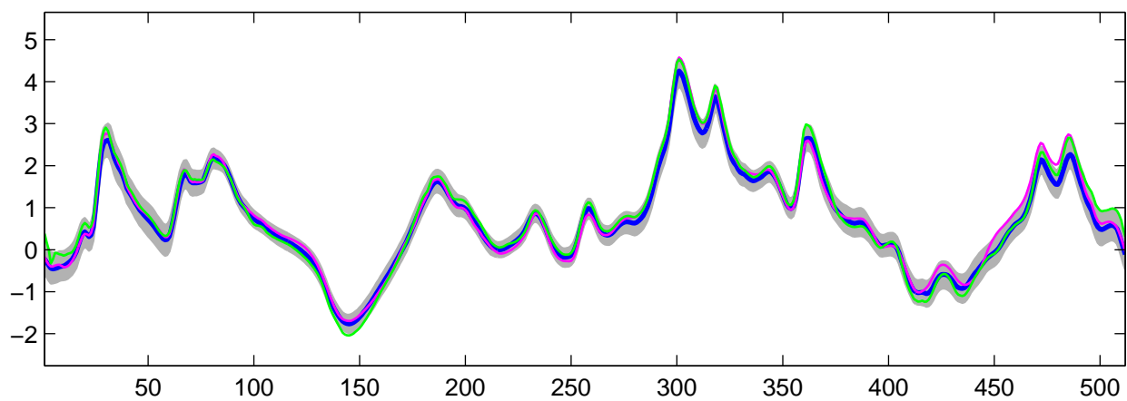
Estimated C_0(t) using R-WFMM: t_3 data, run 1
