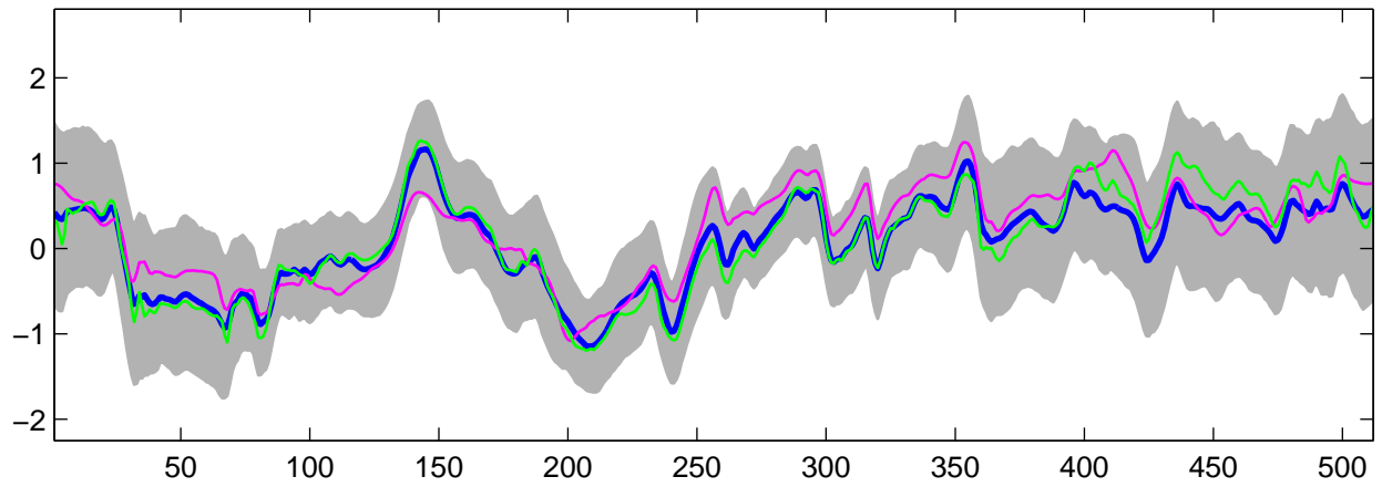
Estimated C_1(t) using G-WFMM: Normal data, run 1
