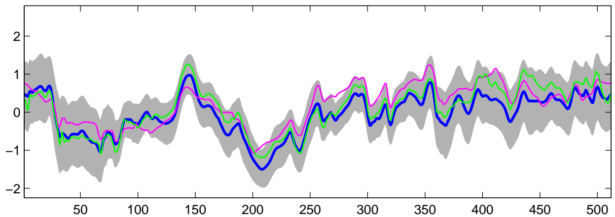
Estimated C_1(t) using R-WFMM: Normal data, run 1
