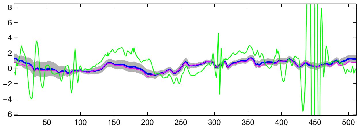
Estimated C_1(t) using R-WFMM: t_1 data, run 1
