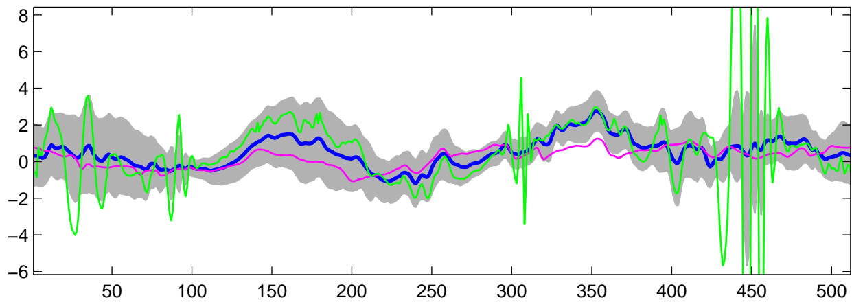
Estimated C_1(t) using G-WFMM: t_1 data, run 1
