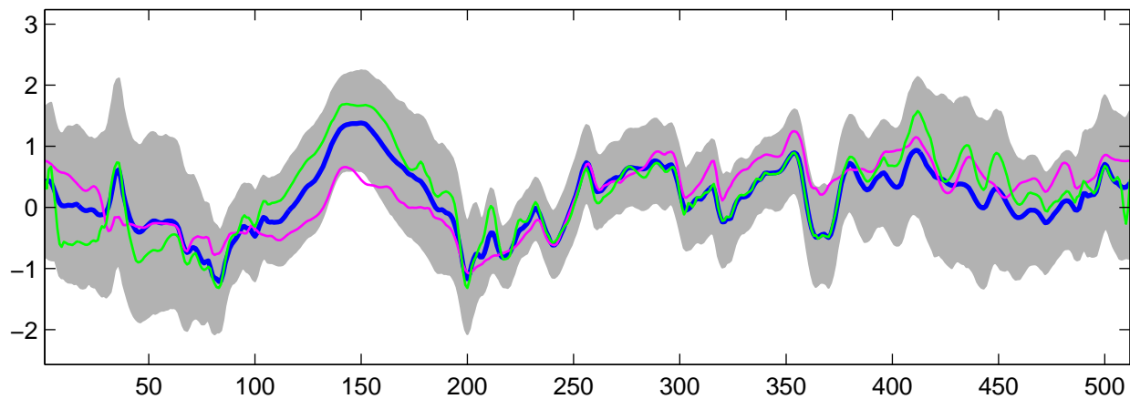
Estimated C_1(t) using G-WFMM: t_2 data, run 1
