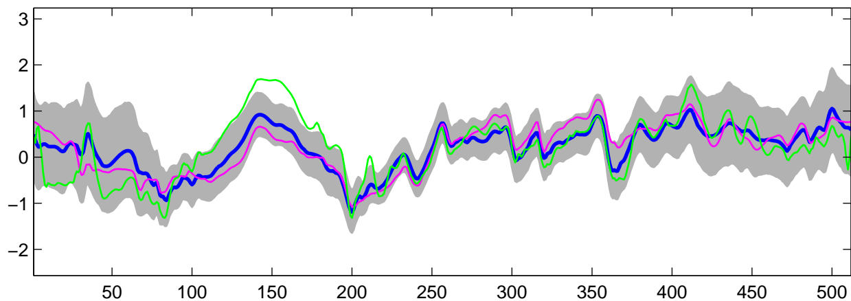
Estimated C_1(t) using R-WFMM: t_2 data, run 1
