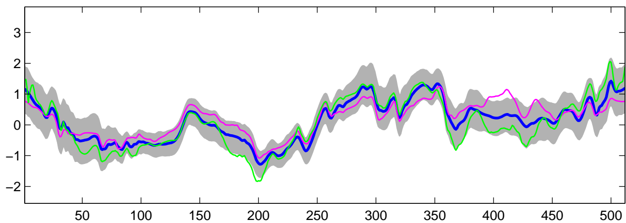
Estimated C_1(t) using R-WFMM: t_3 data, run 1
