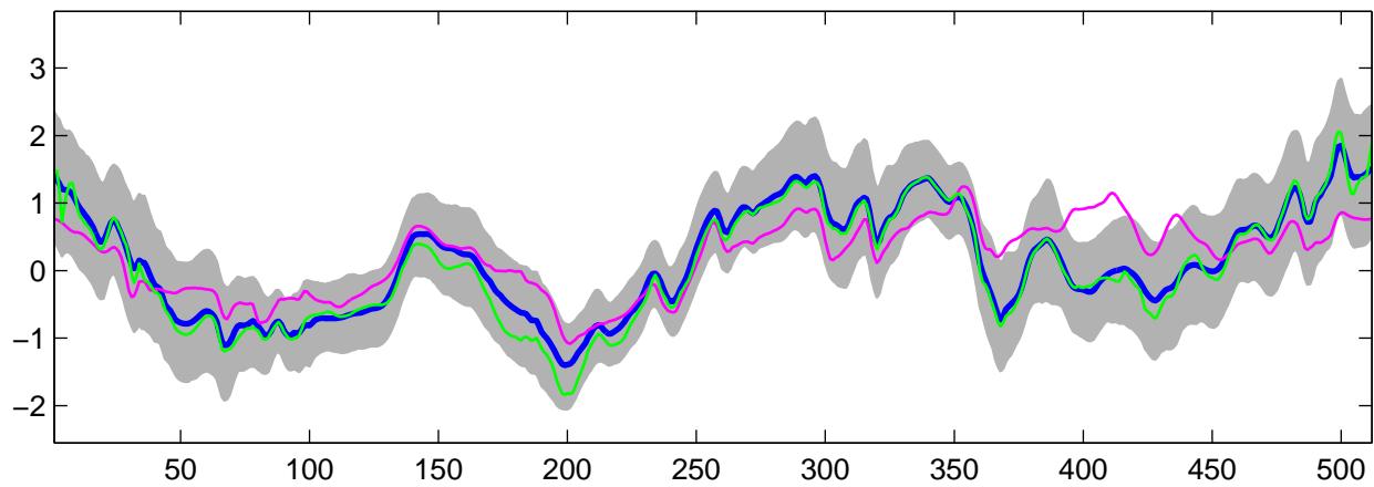
Estimated C_1(t) using G-WFMM: t_3 data, run 1
