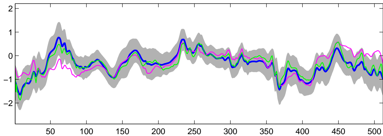
Estimated C_2(t) using R-WFMM: DE data, run 1
