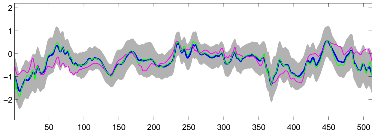
Estimated C_2(t) using G-WFMM: DE data, run 1
