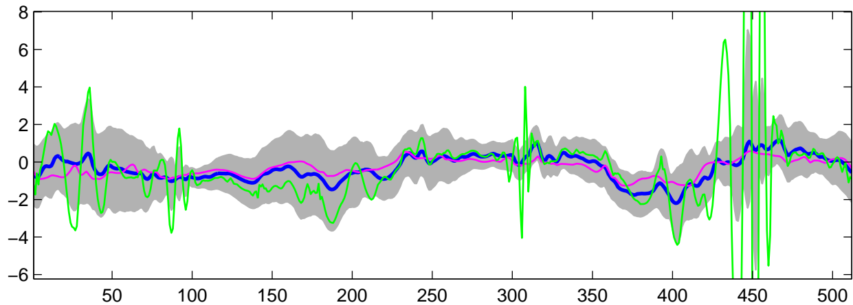
Estimated C_2(t) using G-WFMM: t_1 data, run 1
