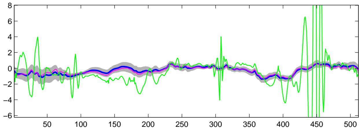
Estimated C_2(t) using R-WFMM: t_1 data, run 1
