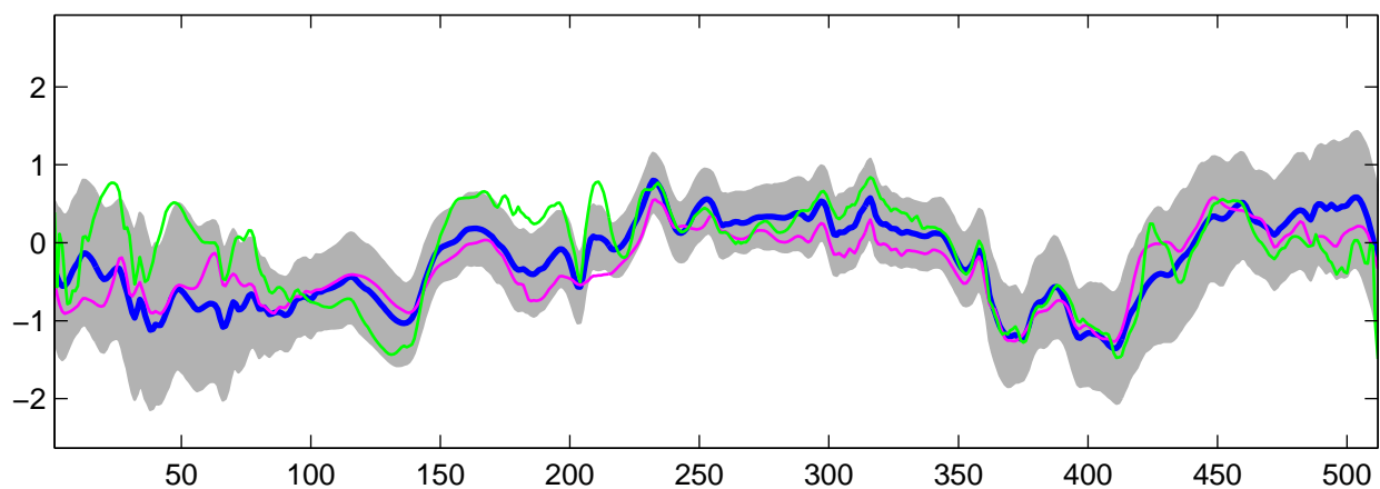
Estimated C_2(t) using R-WFMM: t_2 data, run 1
