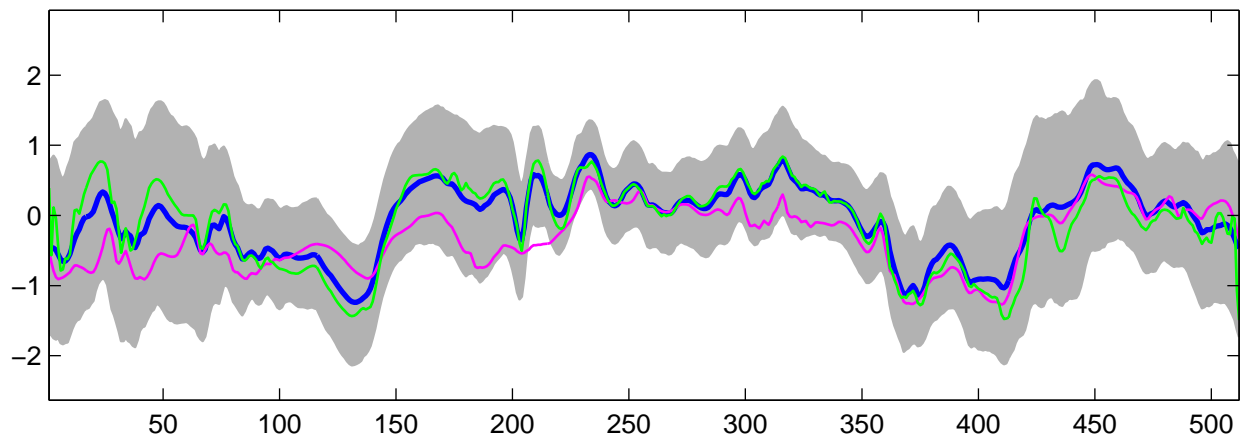
Estimated C_2(t) using G-WFMM: t_2 data, run 1
