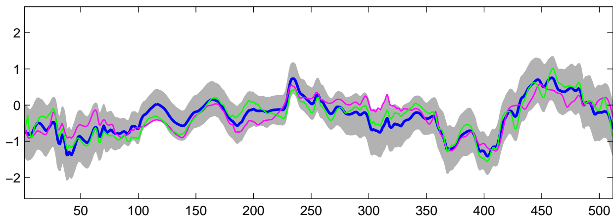
Estimated C_2(t) using R-WFMM: t_3 data, run 1
