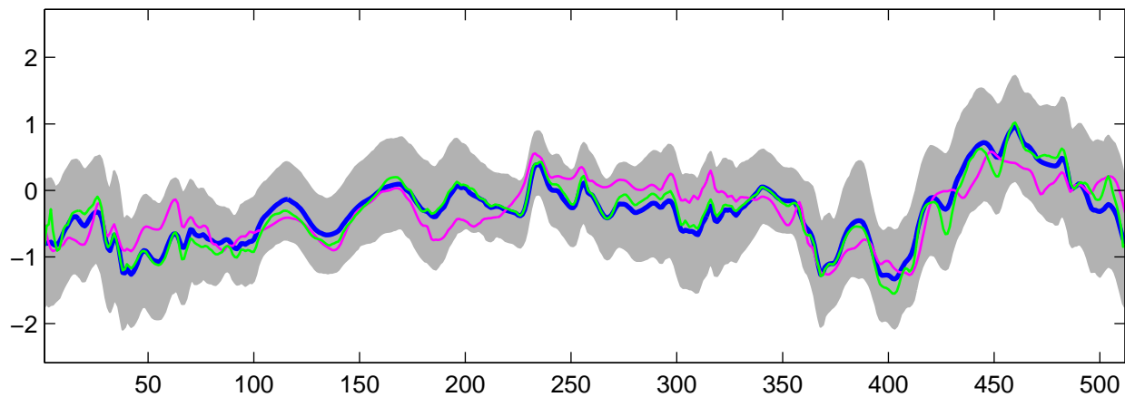
Estimated C_2(t) using G-WFMM: t_3 data, run 1
