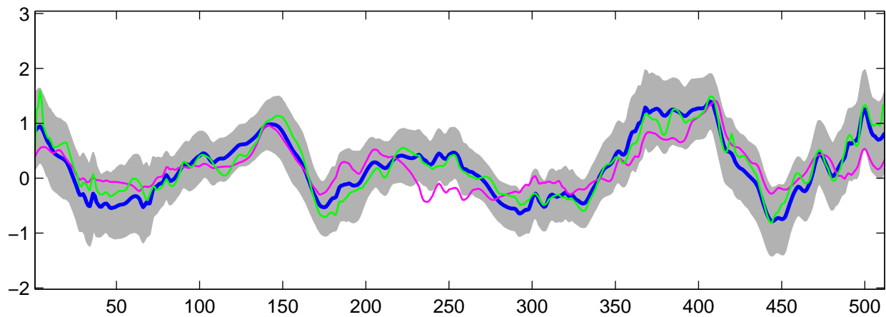
Estimated C_3(t) using R-WFMM: DE data, run 1
