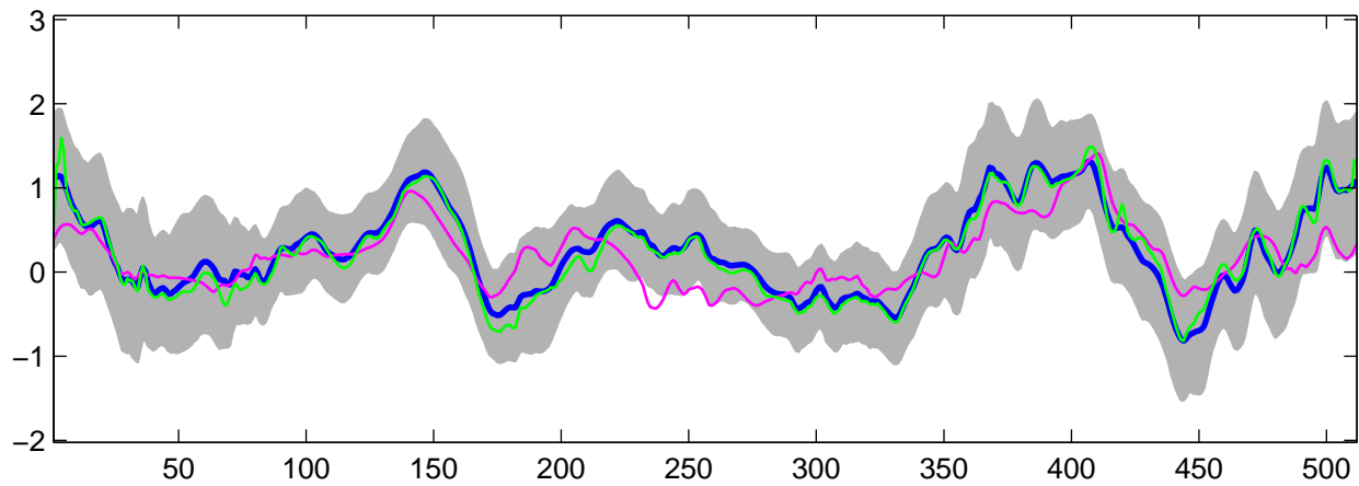
Estimated C_3(t) using G-WFMM: DE data, run 1
