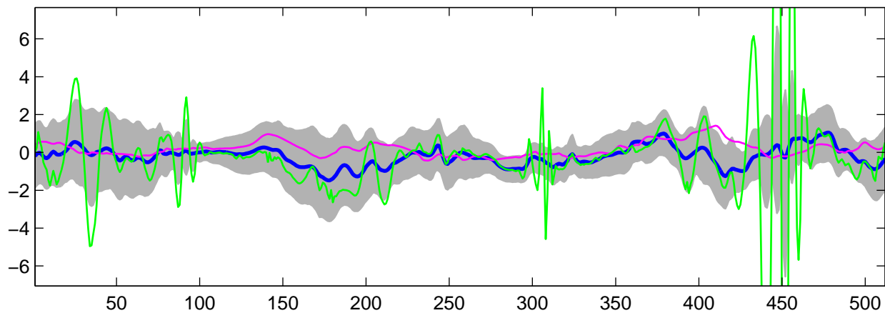
Estimated C_3(t) using G-WFMM: t_1 data, run 1
