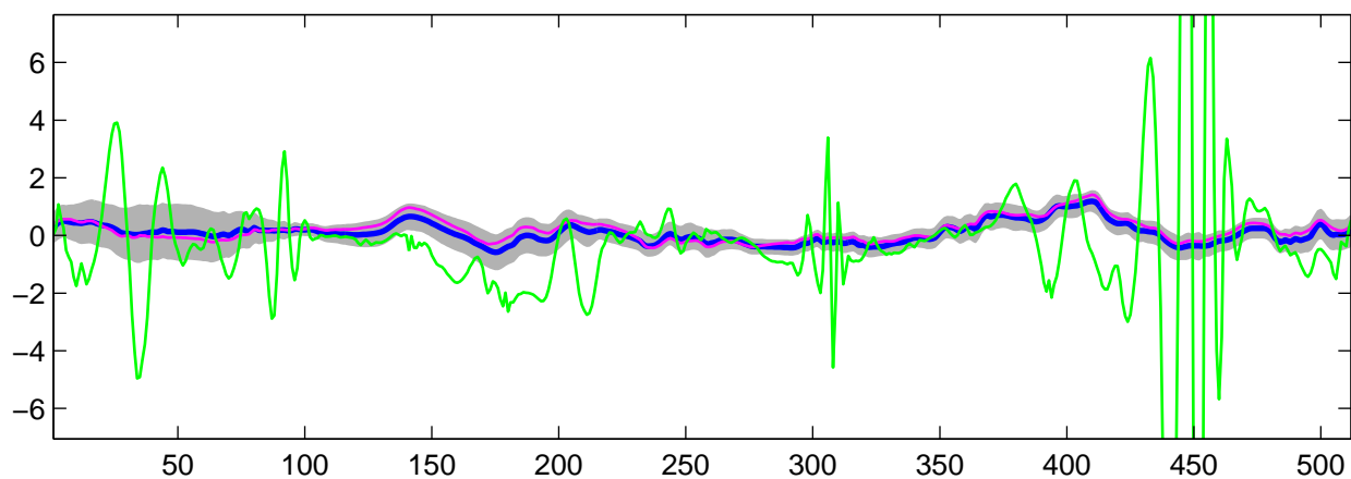
Estimated C_3(t) using R-WFMM: t_1 data, run 1
