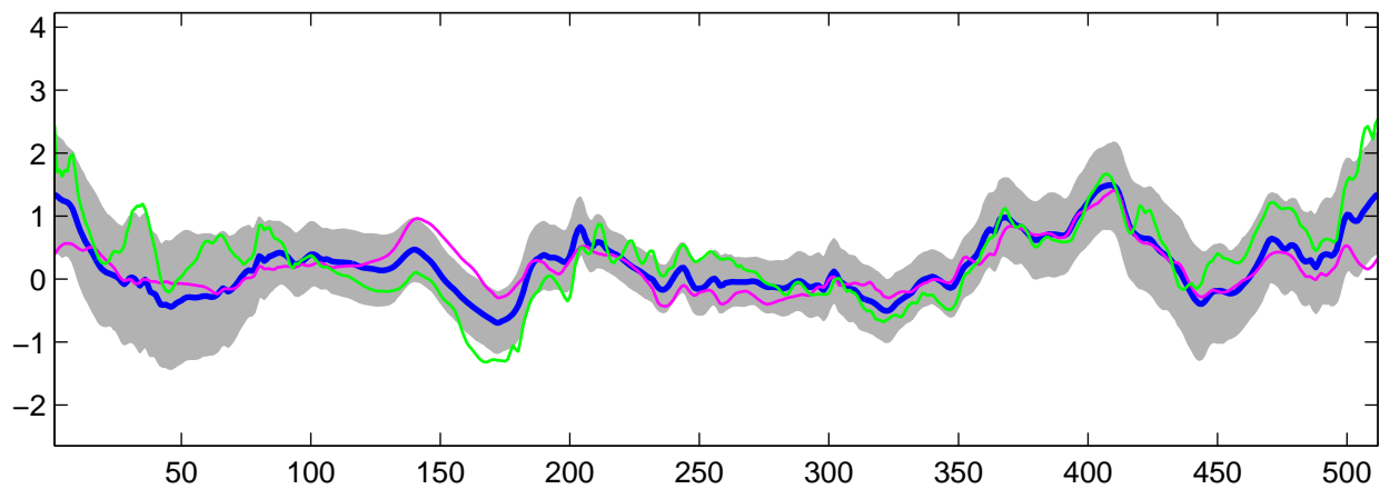
Estimated C_3(t) using R-WFMM: t_2 data, run 1
