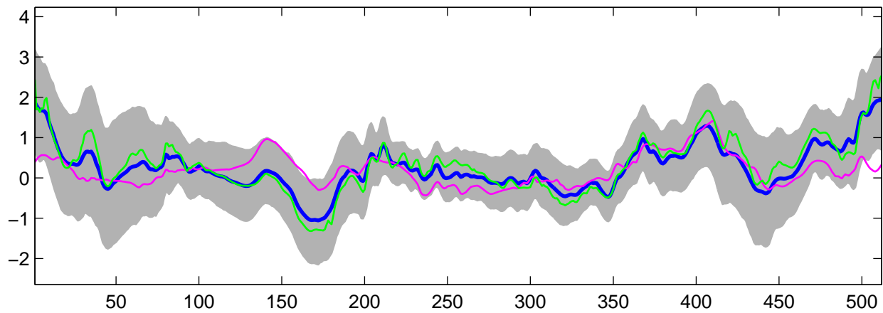
Estimated C_3(t) using G-WFMM: t_2 data, run 1
