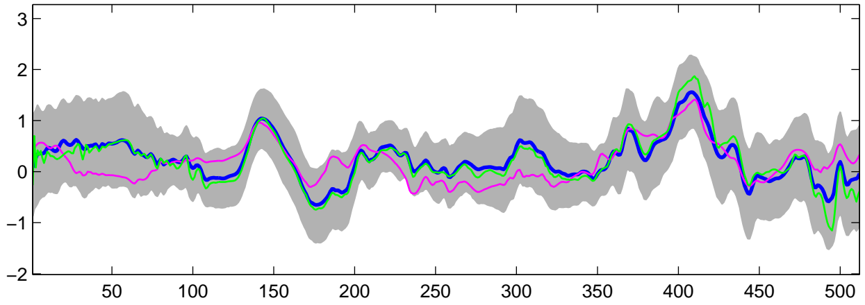
Estimated C_3(t) using G-WFMM: t_3 data, run 1
