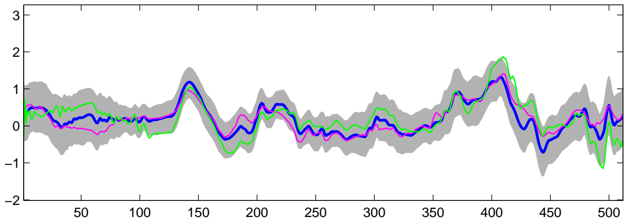
Estimated C_3(t) using R-WFMM: t_3 data, run 1
