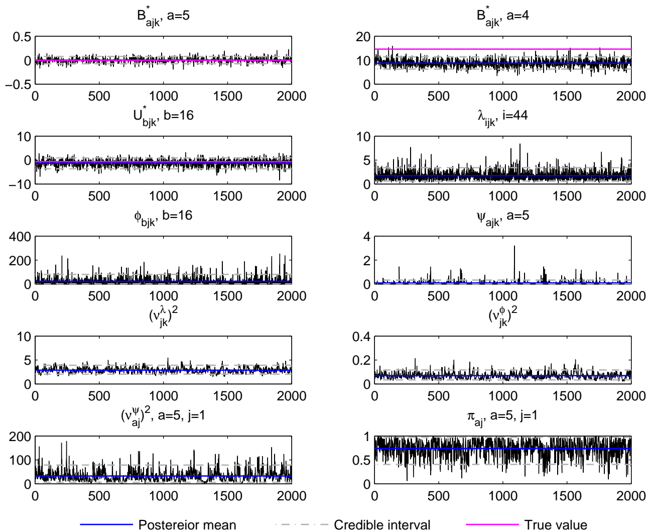
Trace plot, j=1, k=5 , DE data, simulation run 1
