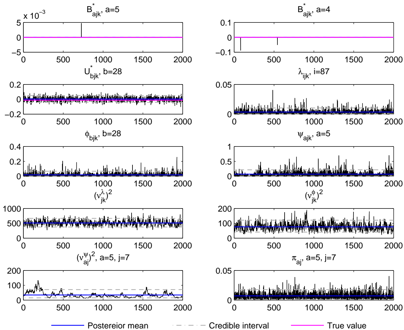
Trace plot, j=7, k=1 , Normal data, simulation run 1
