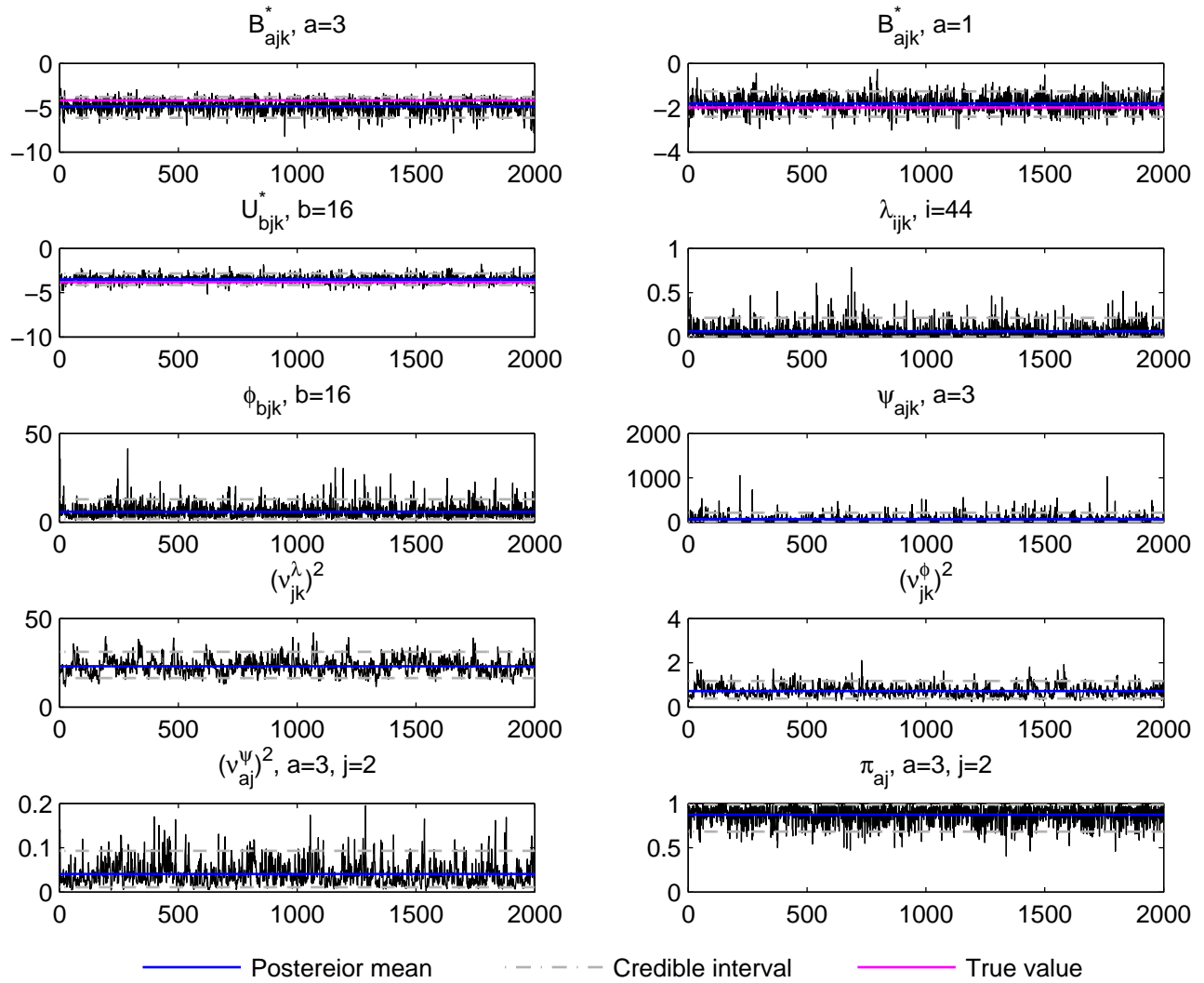
Trace plot, j=2, k=4, t_j data, simulation run 1
