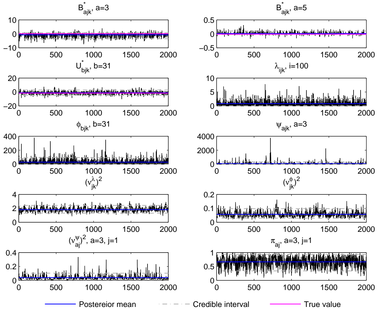
Trace plot, j=1, k=6, t_2 data, simulation run 1
