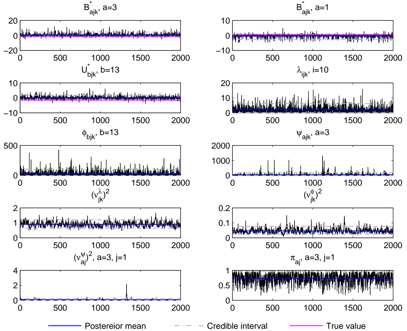
Trace plot, j=1, k=7, t_3 data, simulation run 1
