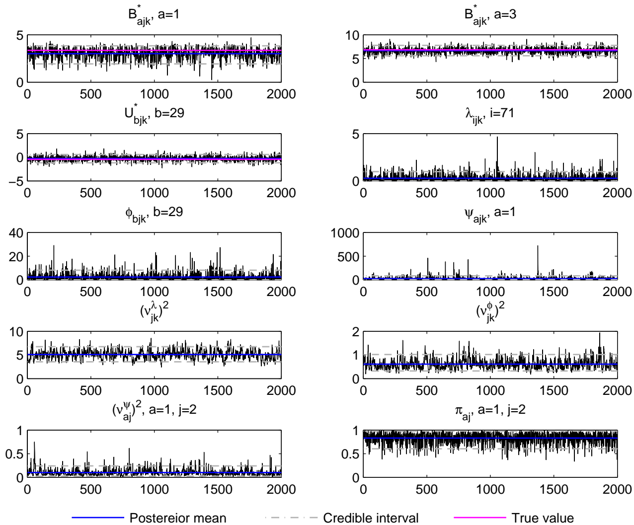
Trace plot, j=2, k=5 , DE data, simulation run 1
