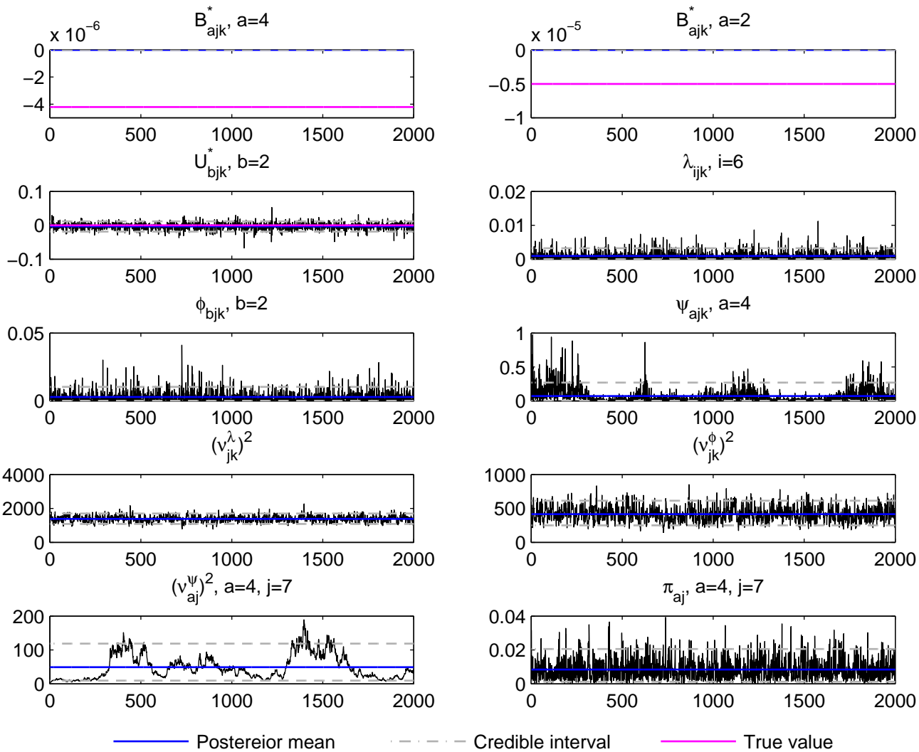
Trace plot, j=7, k=2 , Normal data, simulation run 1
