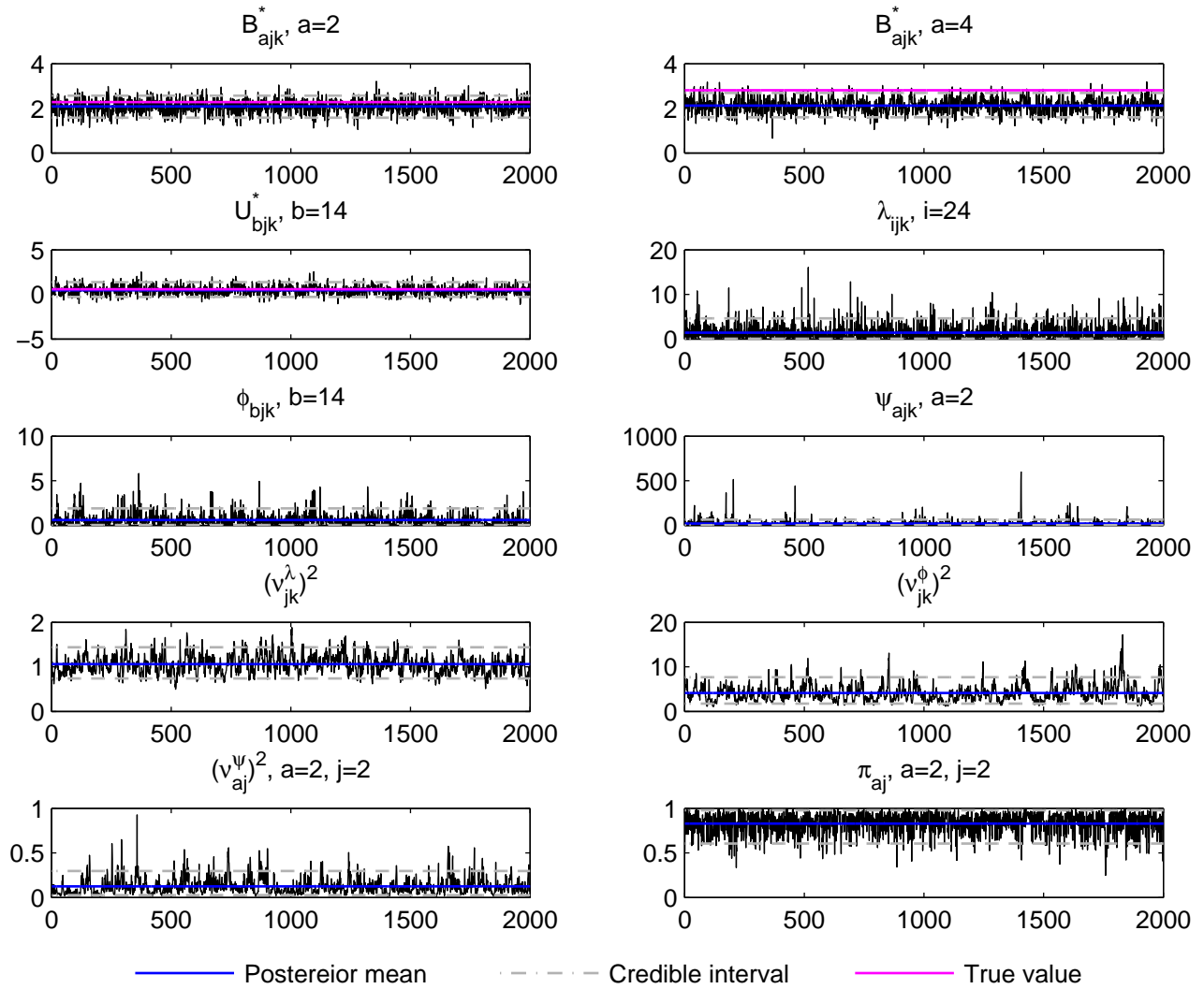
Trace plot, j=2, k=6, t_2 data, simulation run 1
