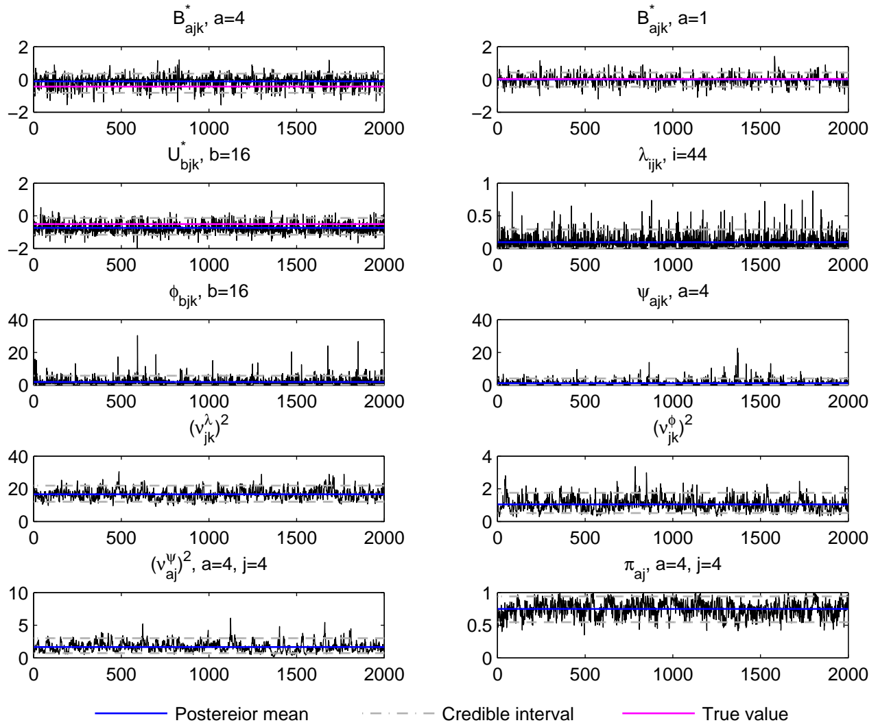
Trace plot, j=4, k=1, t_3 data, simulation run 1
