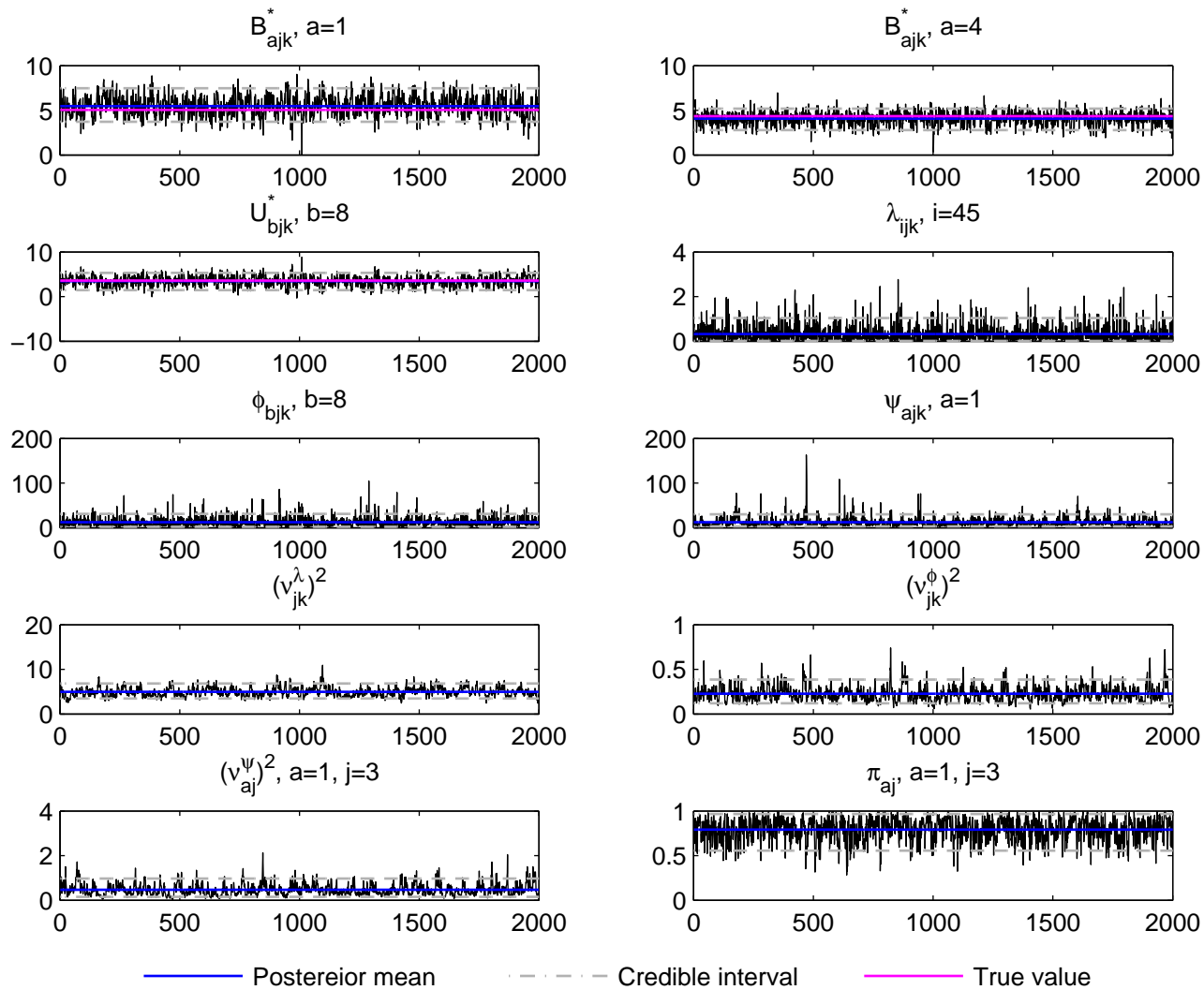
Trace plot, j=3, k=1 , DE data, simulation run 1
