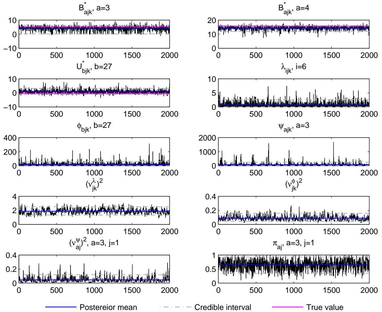
Trace plot, j=1, k=2, t_j data, simulation run 1
