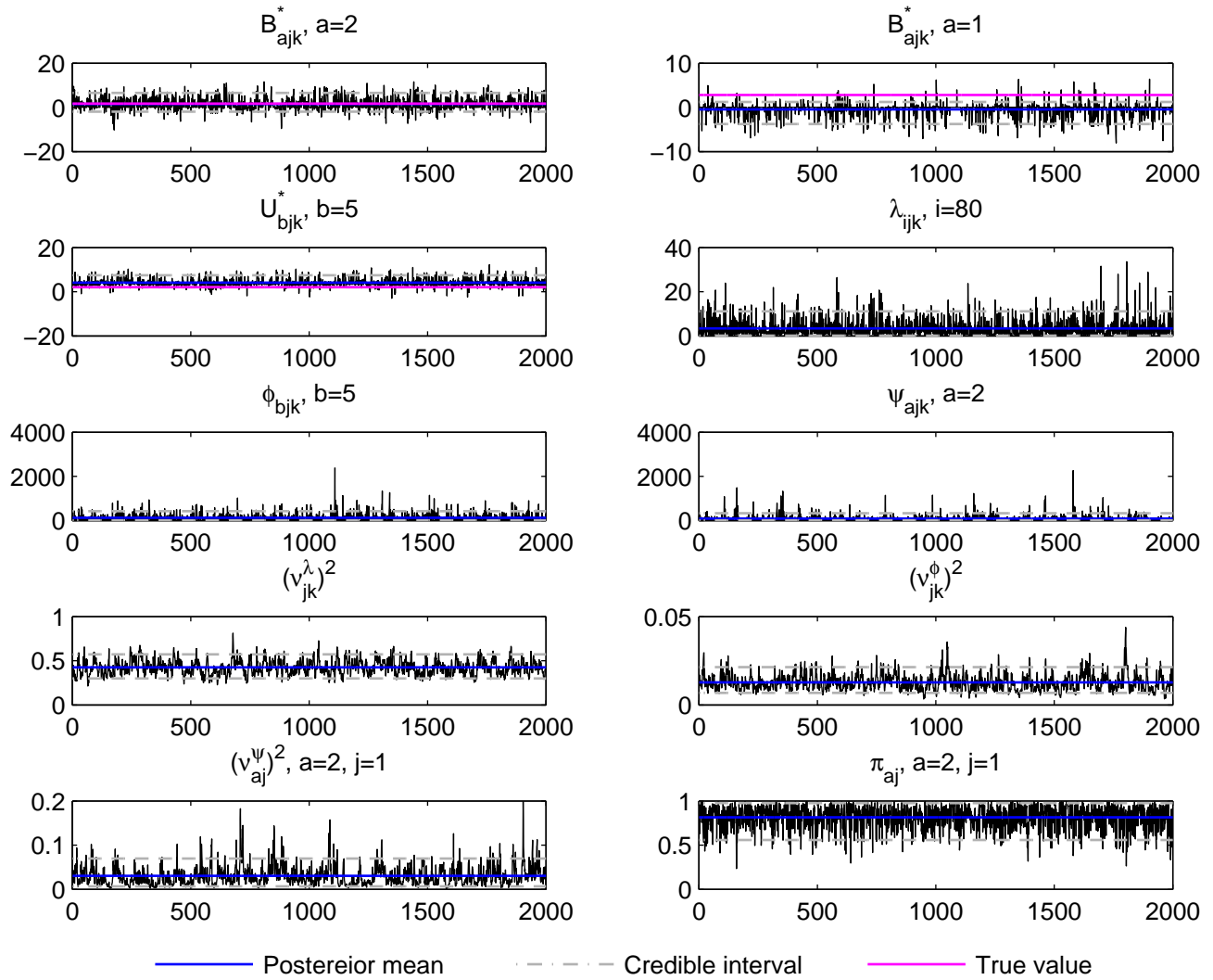
Trace plot, j=1, k=3, t_2 data, simulation run 1
