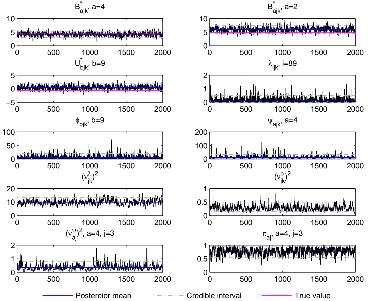
Trace plot, j=3, k=1, t_3 data, simulation run 1
