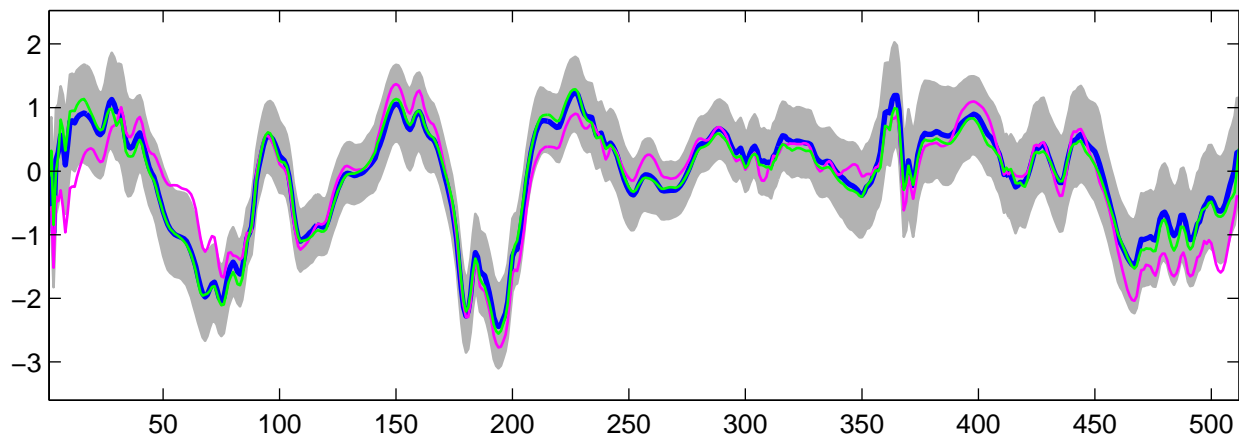
Estimated U_{10}(t) using G-WFMM: DE data, run 1
