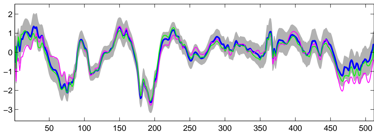
Estimated U_{10}(t) using R-WFMM: DE data, run 1
