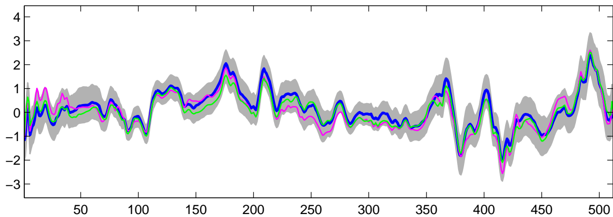
Estimated U_{10}(t) using R-WFMM: Normal data, run 1
