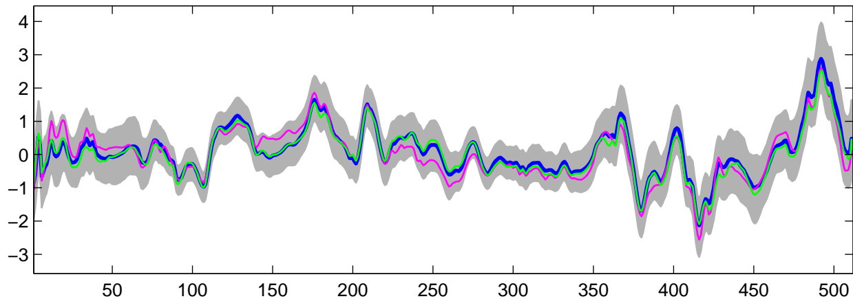
Estimated U_{10}(t) using G-WFMM: Normal data, run 1
