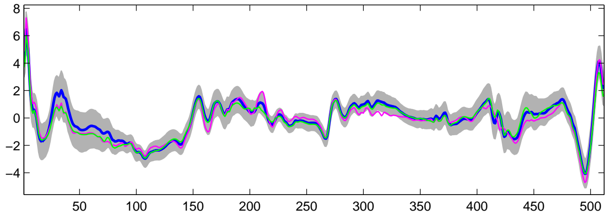
Estimated U_{10}(t) using G-WFMM: t_2 data, run 1
