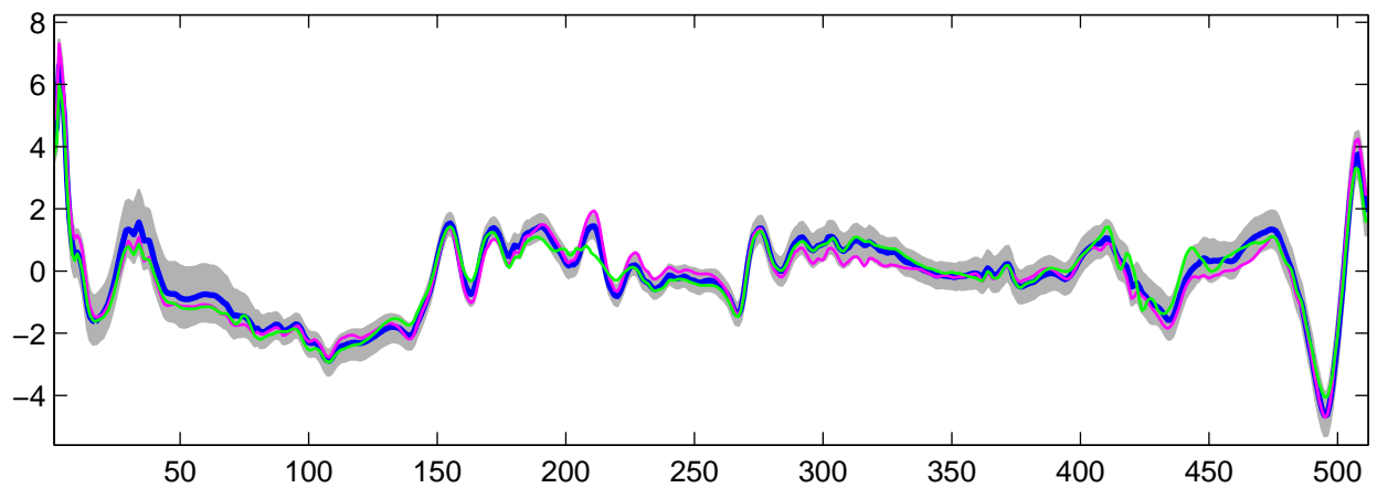
Estimated U_{10}(t) using R-WFMM: t_2 data, run 1
