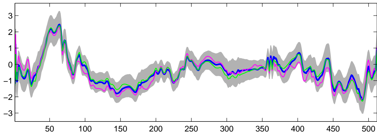
Estimated U_{10}(t) using G-WFMM: t_3 data, run 1
