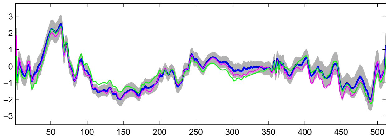
Estimated U_{10}(t) using R-WFMM: t_3 data, run 1
