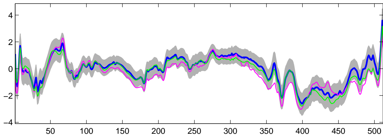
Estimated U_{11}(t) using R-WFMM: Normal data, run 1
