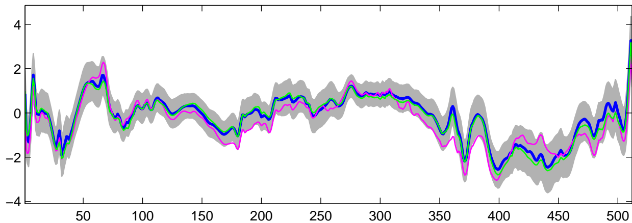
Estimated U_{11}(t) using G-WFMM: Normal data, run 1
