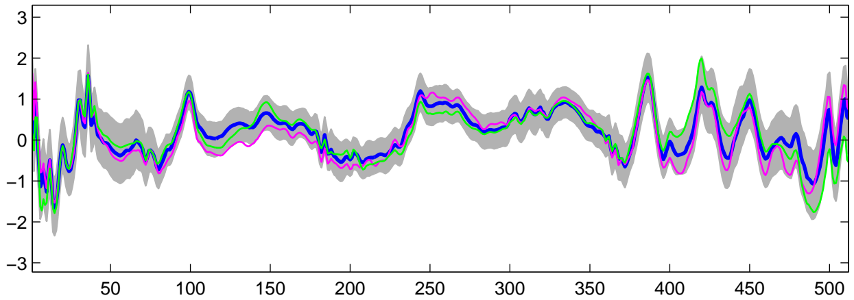
Estimated U_{11}(t) using R-WFMM: t_3 data, run 1
