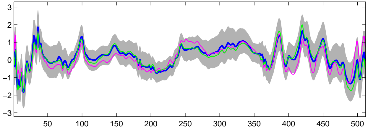
Estimated U_{11}(t) using G-WFMM: t_3 data, run 1
