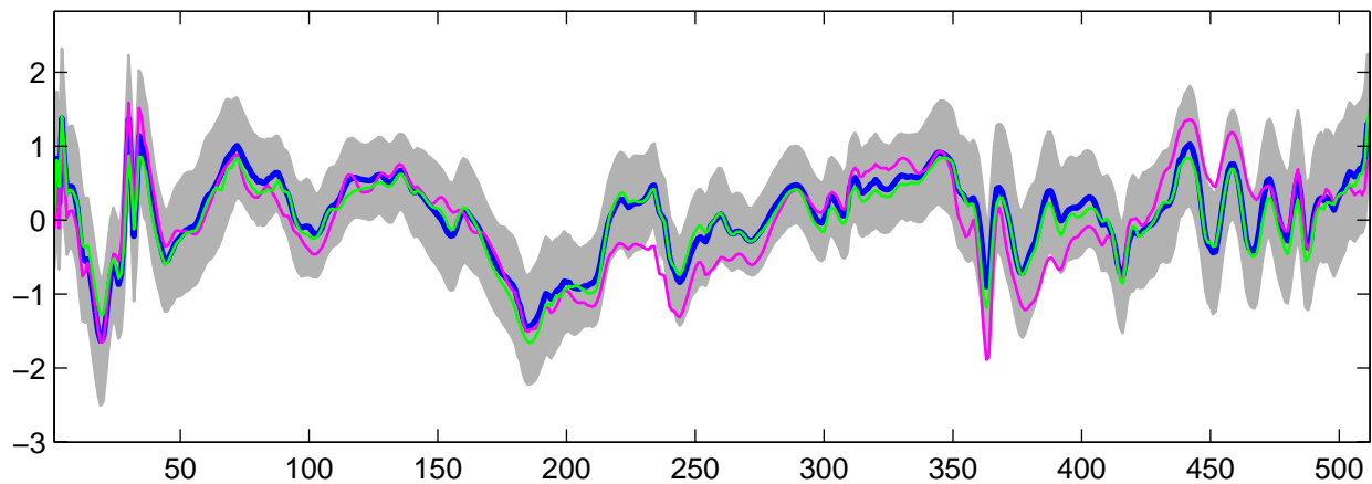
Estimated U_{12}(t) using G-WFMM: DE data, run 1
