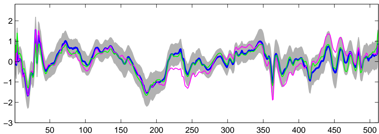
Estimated U_{12}(t) using R-WFMM: DE data, run 1
