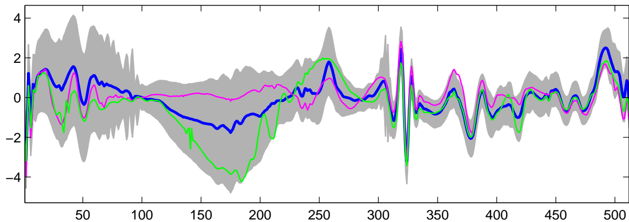
Estimated U_{12}(t) using G-WFMM: t_1 data, run 1
