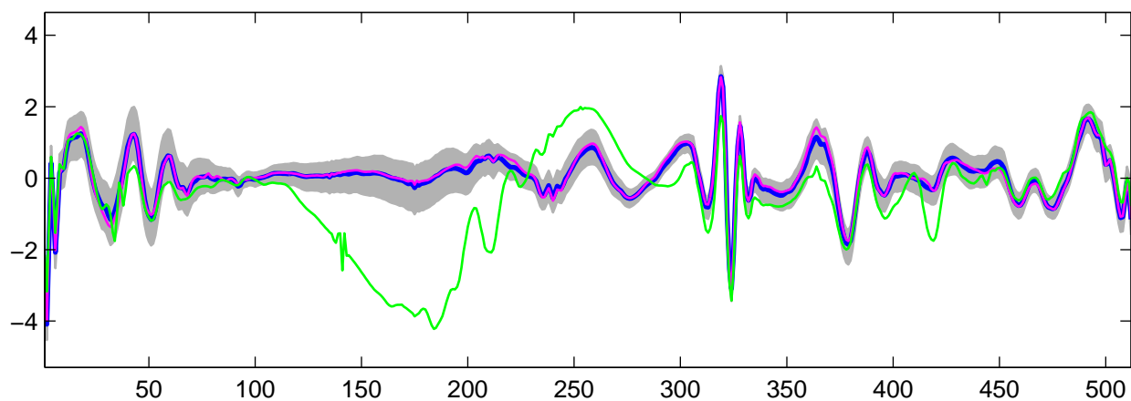
Estimated U_{12}(t) using R-WFMM: t_1 data, run 1
