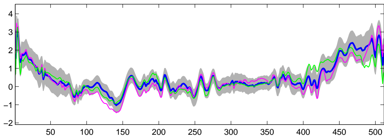
Estimated U_{12}(t) using R-WFMM: t_3 data, run 1
