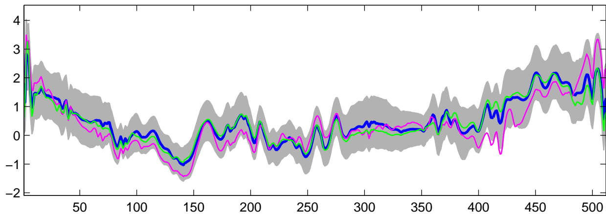
Estimated U_{12}(t) using G-WFMM: t_3 data, run 1
