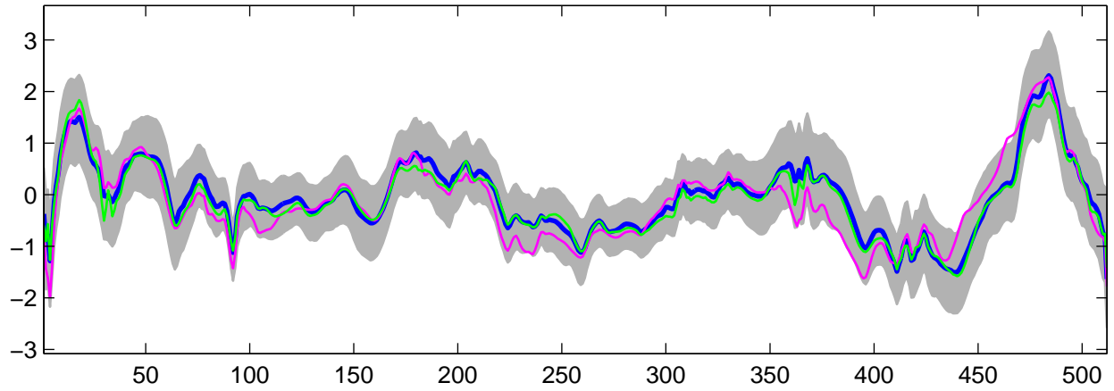
Estimated U_{13}(t) using G-WFMM: DE data, run 1
