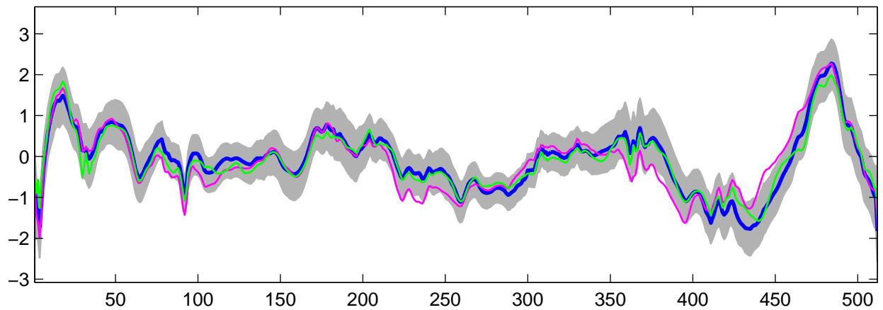
Estimated U_{13}(t) using R-WFMM: DE data, run 1
