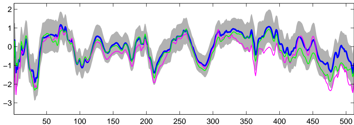
Estimated U_{13}(t) using R-WFMM: Normal data, run 1
