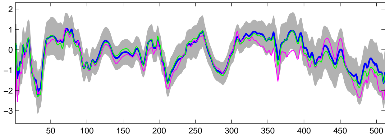
Estimated U_{13}(t) using G-WFMM: Normal data, run 1
