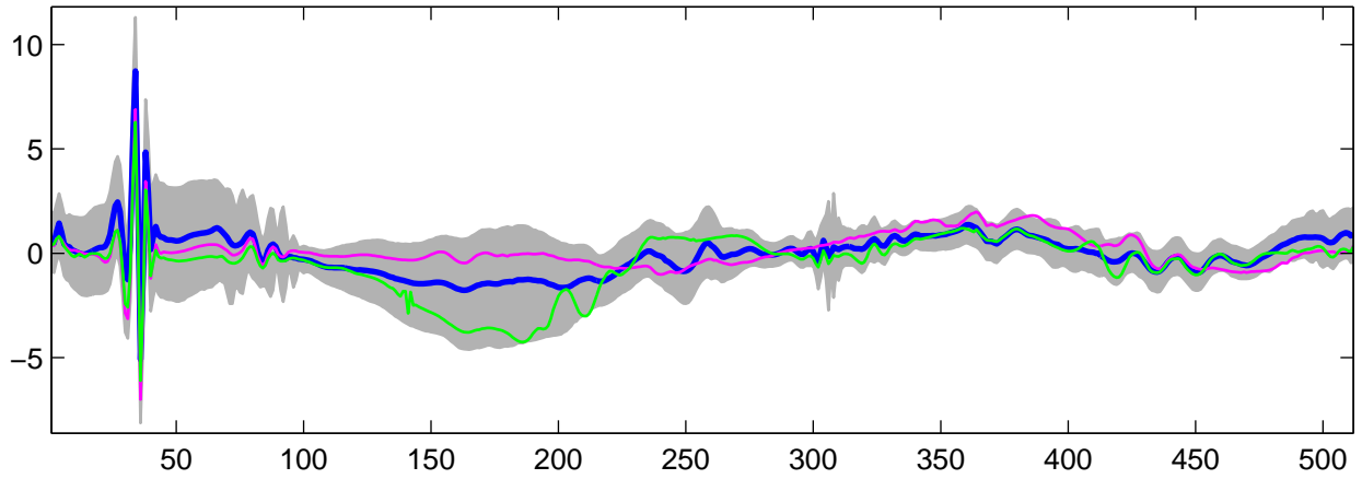
Estimated U_{13}(t) using G-WFMM: t_1 data, run 1
