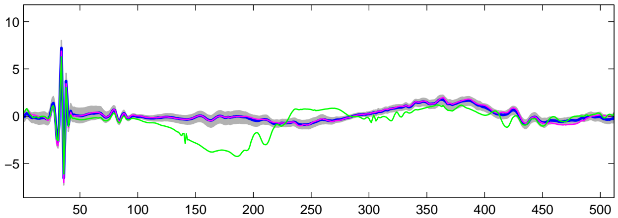
Estimated U_{13}(t) using R-WFMM: t_1 data, run 1
