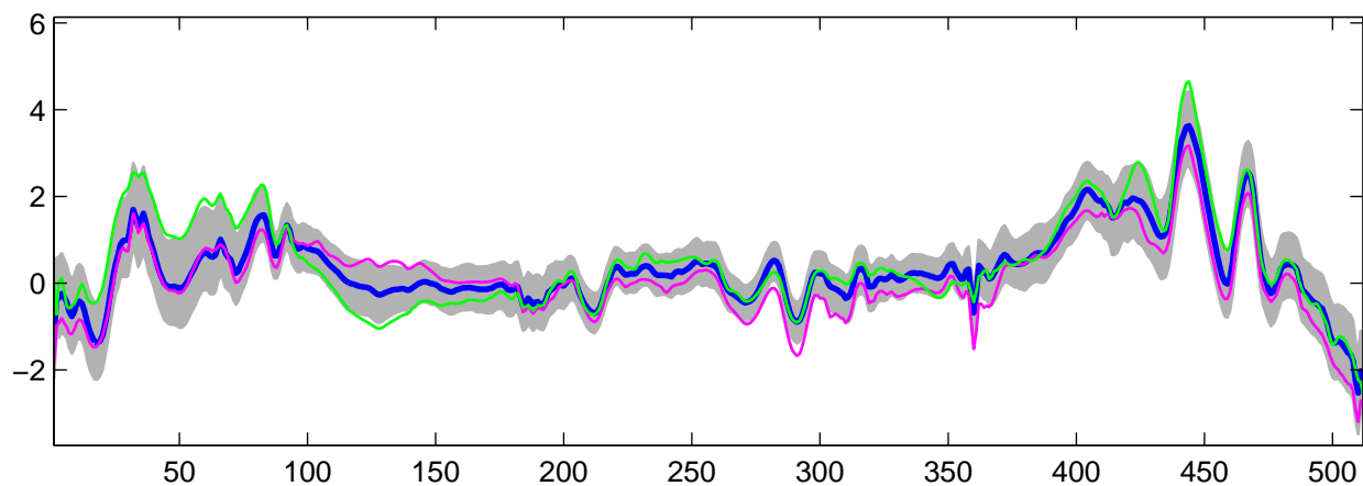
Estimated U_{13}(t) using R-WFMM: t_2 data, run 1
