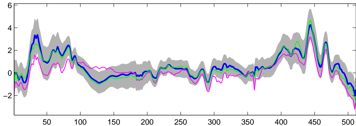
Estimated U_{13}(t) using G-WFMM: t_2 data, run 1
