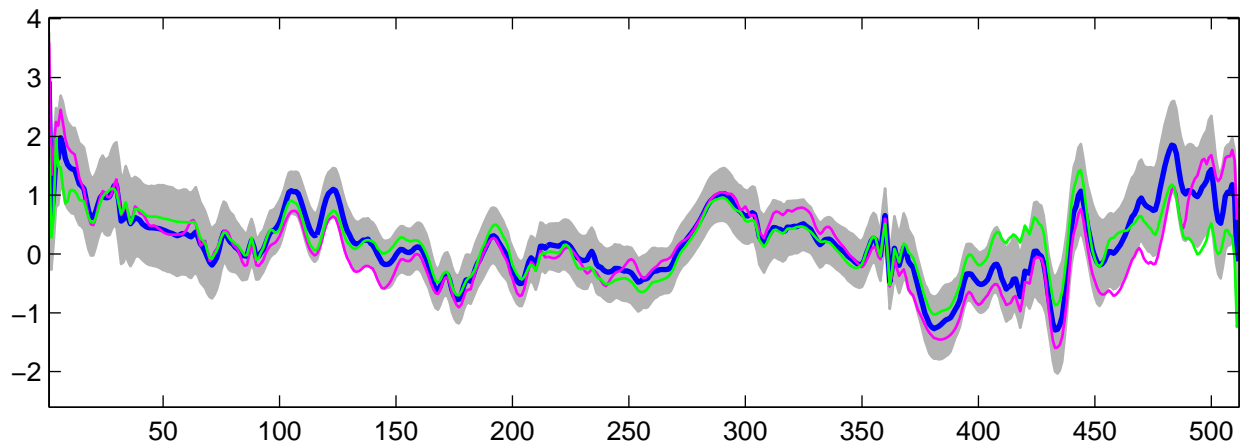
Estimated U_{13}(t) using R-WFMM: t_3 data, run 1
