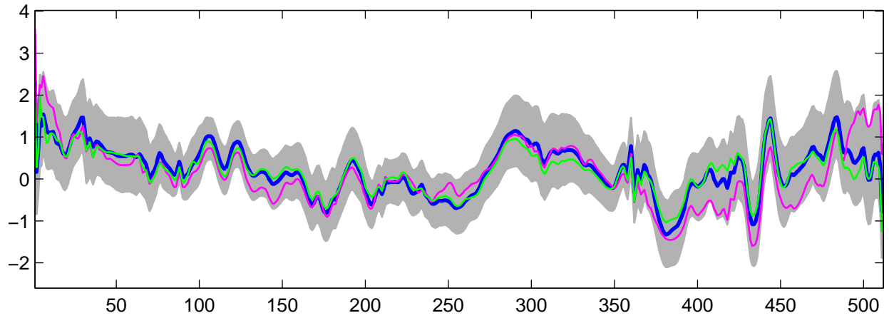
Estimated U_{13}(t) using G-WFMM: t_3 data, run 1
