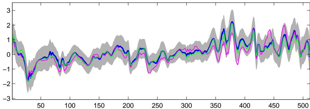
Estimated U_{14}(t) using G-WFMM: DE data, run 1
