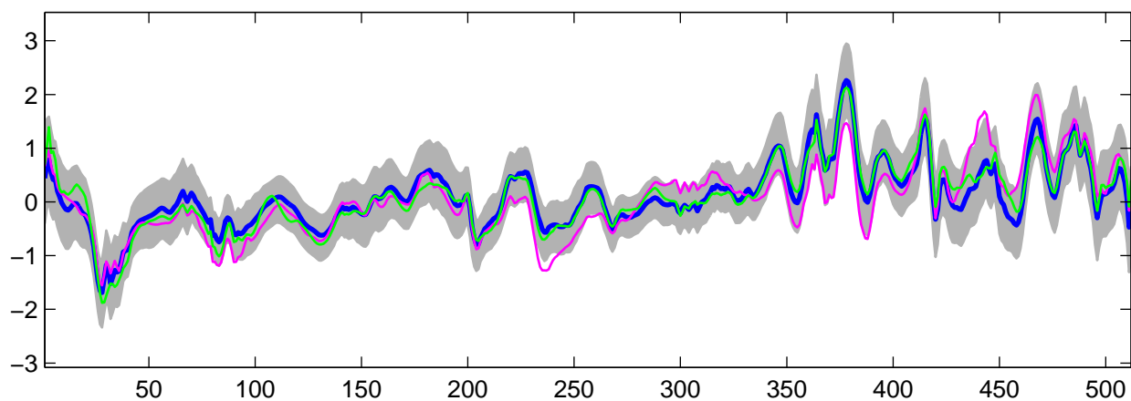
Estimated U_{14}(t) using R-WFMM: DE data, run 1
